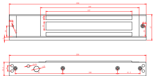
280KG Magnetic Lock
