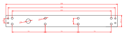
Mounting Plate for 280KG Magnetic Lock
