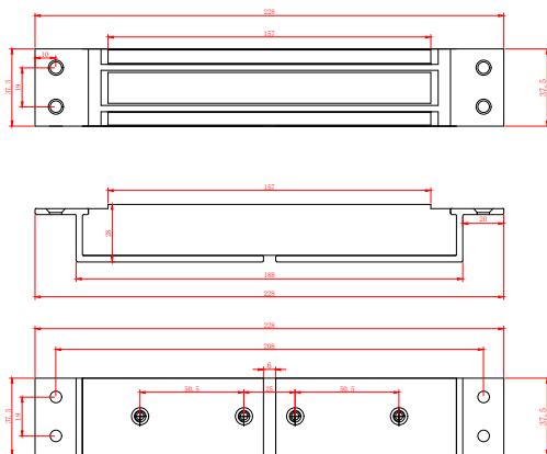
280KG Mortise Mount Magnetic Lock Frameless
