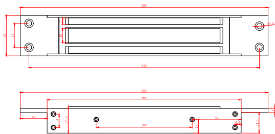
280KG Mortise Mount Magnetic Lock
